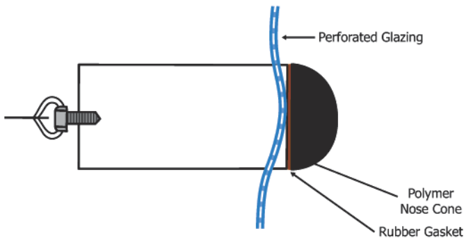
FIG. 12 Diagram of Impactor Perforating the Glazing Panel with the Entire Gasket Visible (Fail)
